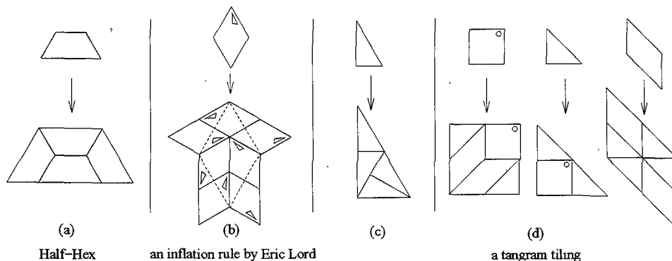
Figure 2: Four inflation rules for nonperiodic tilings.
