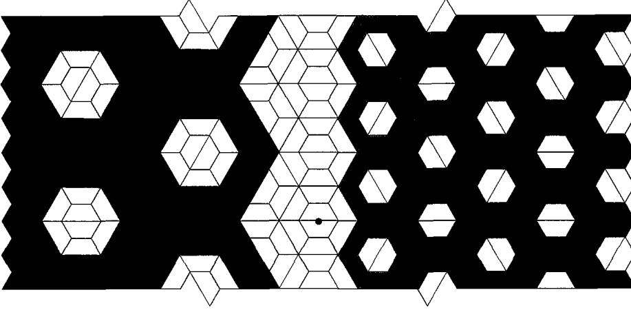
Figure 3: Periodic structures in a nonperiodic tiling
