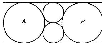
Figure 8: t_{AB}^2 = 8ab
