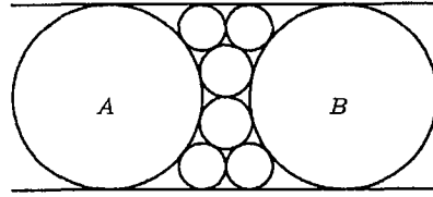
Figure 9: t_{AB}^2 = (25/4) \cdot ab
