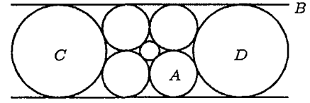
Figure 10: t_{AB}^2 = 8ab , t_{CD}^2 = (4\sqrt{2} + 9)cd
