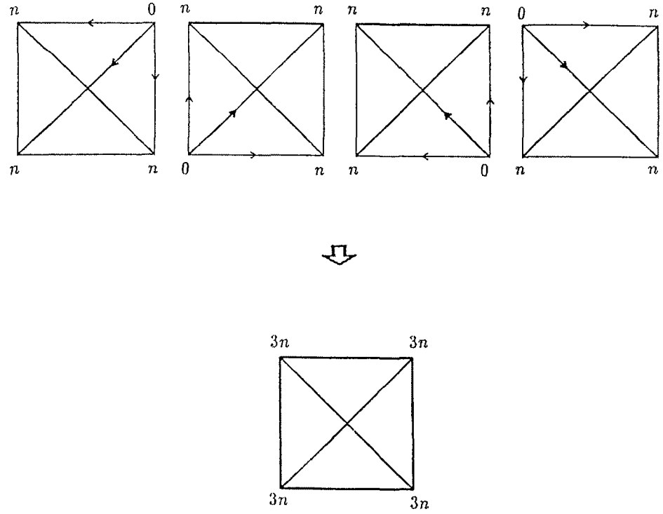
Figure 3: Regular tetrahedra ( \alpha_1 ) operated on by 0, \phi_3, 2\phi_3, 3\phi_3 rotations ( \cos \phi_3 = -1/3 ) and superposed \alpha_1 with homogeneous density 3n . A sense of stacking layers of regular triangle ( \alpha_2 ), with increment weight is denoted by arrows
