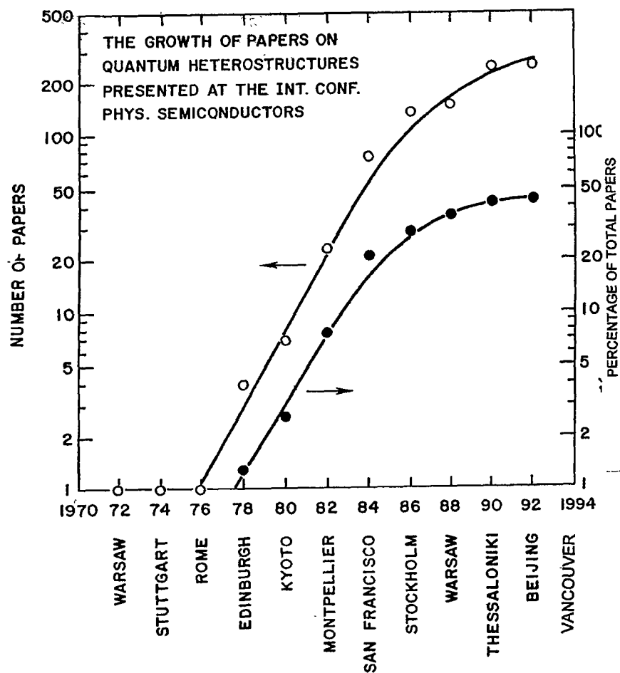
Figure 3: Growth in relevant papers in the biennial International Conference on the Physics of Semiconductors.
