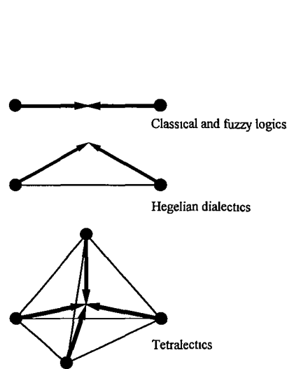
Figure 1: A possible representation of the classical and fuzzy logics, Hegelian dialectics and tetralectics.
