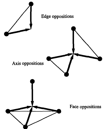
Figure 2: Different classes of oppositions in tetralectics.
