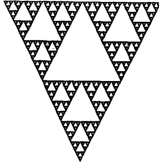
Figure 4a: Simulation of hyperincursive equation 4 with initial condition 4a.
