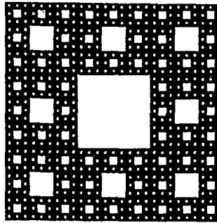
Figure 5a: Simulation of hyperincursive equation (5) giving a square fractal.
