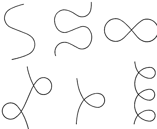
Figure 2: Euler's Elastica.
