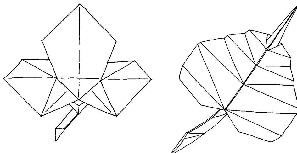
Figure 13: Maple leaf has bilateral symmetry.
