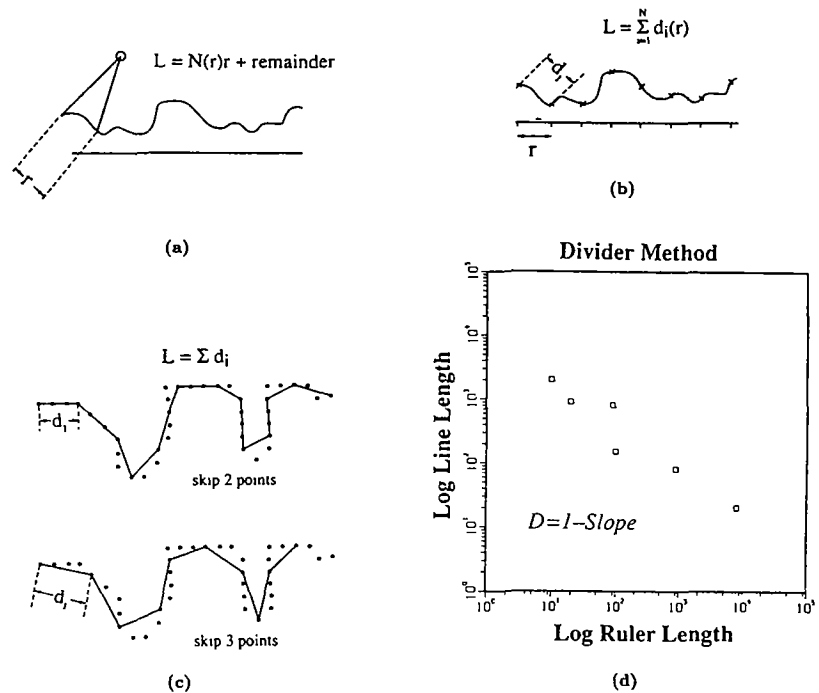
Figure 2: (a) Divider (ruler) method: caliper or divider applied to surface of profile; (b) modified divider where straight line length between divisions along base are measured; (c) digitized ruler method using point counting (Clark, 1986); (d) example of plotted measurements where D = 1 - \text{slope} .
