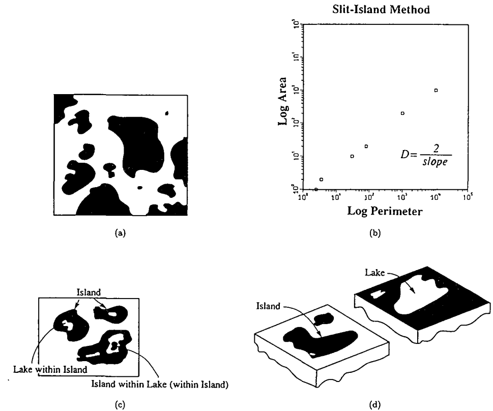
Figure 5: Slit-Island method: (a) take a horizontal cut through the surface creating islands (dark regions); (b) example of log-log plot where D = 2/\text{slope} ; (c) Mandelbrot's "island within lakes"; (d) Huang et al. 's "islands within lakes".
