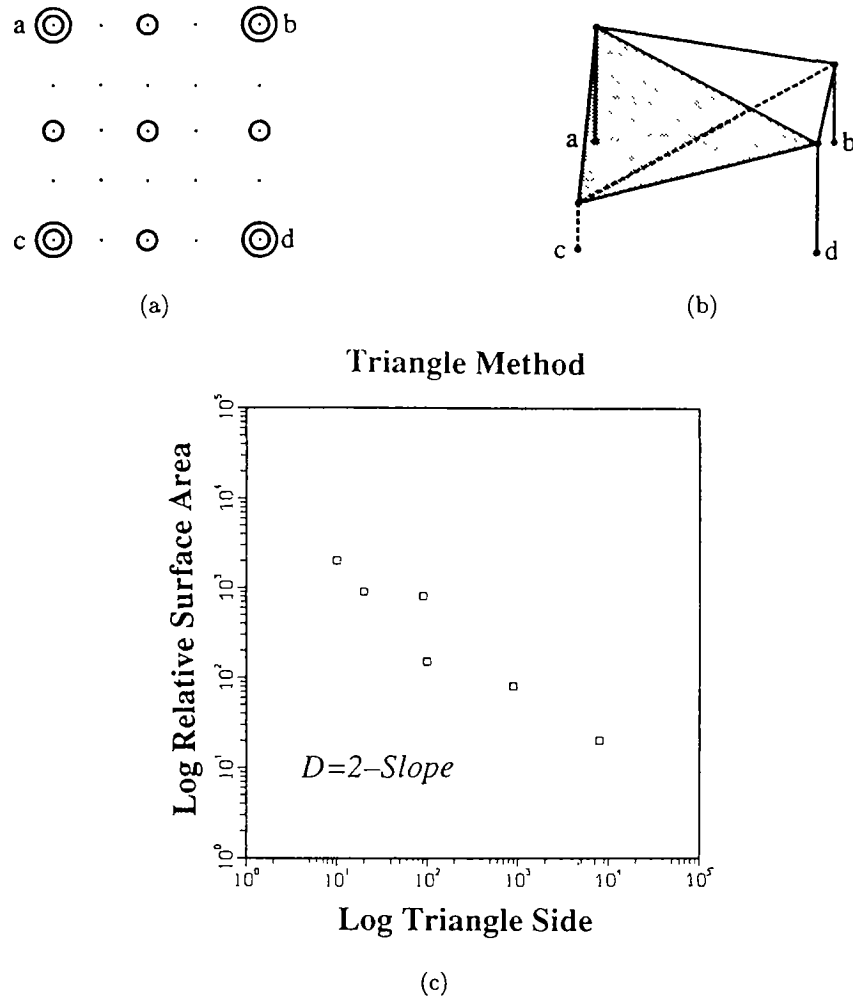
Figure 4: Triangle method: (a) plan view of surface covered with triangles of consecutively smaller size; (b) choice of diagonal may give different surface area, solid diagonal gives ridge while dashed diagonal gives valley; (c) example of log-log plot where D = 2 - \text{slope} ; A is area of rough triangle; A_0 is area of flat triangle; Relative surface area is A/A_0 , (after Denley, 1990).
