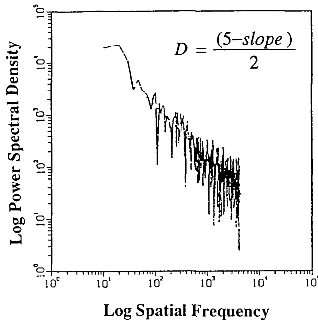
Figure 6: Power spectral method: compute spectral density of profile as a function of frequency and plot on log-log graph; D = (5 - \text{slope})/2 .
