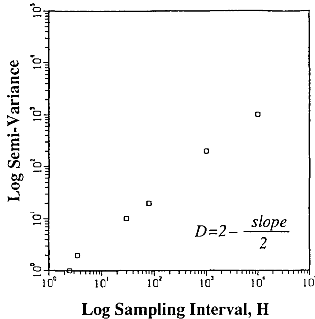
Figure 7: Variogram method: compute semi-variance as a function of sampling interval and plot on log-log graph where D = 2 - (\text{slope}/2) .
