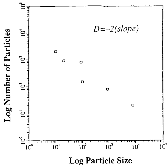
Figure 8: Distribution method: determine the size distribution and plot the log of the size class versus the log of the number of counted objects which are greater than the size class; D = -2 slope, if the size is an area.
