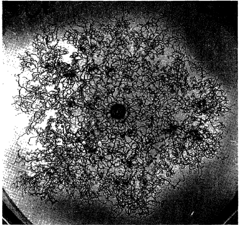
Figure 6a: Example of pattern observed during growth of phase C (the chiral phase).
