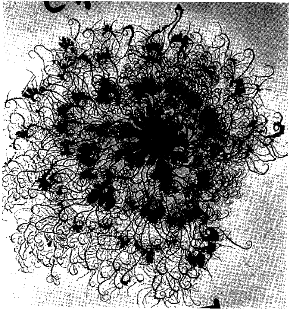
Figure 6b: Example of pattern observed during growth of phase C (the chiral phase).
