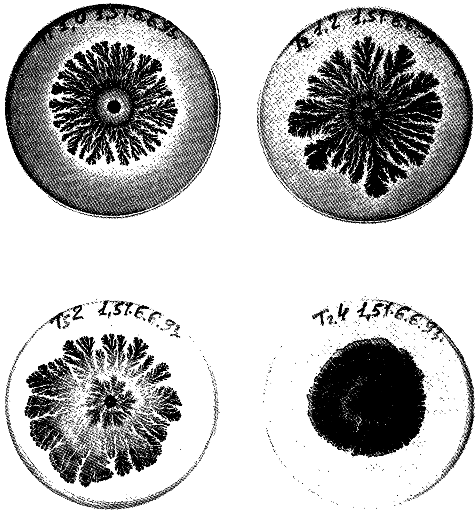
Figure 1: Observed patterns of phase T grown on 1.5 per cent agar concentration. The pepton level is 1g/l, 1.2g/l, 2g/l, and 4g/l for (a), (b) (c) and (d) respectively. At high pepton level the branches are wide, the pattern is very reminiscent of Hele-Shaw patterns (Ben-Jacob and Garik, 1990) and the fractal dimension is close to two. As the pepton level is decreased, the patterns become more ramified similar to DLA simulations.
