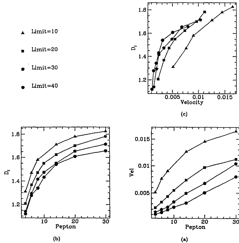
Figure 5. (a) Growth velocity versus food concentration for different N_c . The velocity increases as more food is available for the walkers. As N_c increases, it is harder for the colony to advance and the growth velocity decreases. In all cases the velocity appears to be a smooth function of the growth parameters. (b) The fractal dimension (of mass distribution) versus food concentration for different N_c . The patterns are more compact for high pepton level. (c) The fractal dimension versus growth velocity. A high correlation is observed between these two observable.
