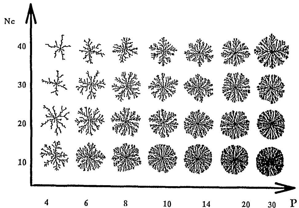
Figure 4: Morphology diagram of the 'communication walkers' model. D = 1.4 , dt = 0.4 , dx = 1 , food consumption per second = 0.04, divide at threshold = 1.0, maximal jump for a walker = 0.2, e = 0.2 , initial radius of colony = 3, initial number of walkers = 20. In the late stage growth the number of walkers is about 10^2 . P (represents the pepton level) is the initial concentration measured in units of the threshold.
