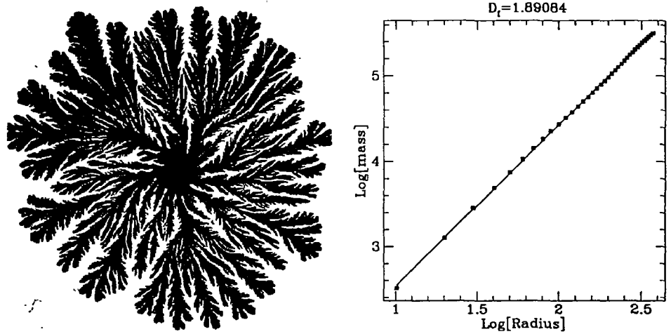
Figure 2: A typical tip-splitting growth and its fractal dimension. In order to perform this calculation, the bacterial colony shape was digitized. The fractal dimension, D_f , is defined such that m \sim r^{D_f} , where m is the mass of the cluster whose distance from the center of the colony is less than r . The fractal dimension was measured using Log-Log plot of the mass distribution vs. cluster radius.
