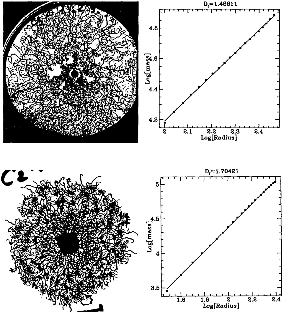
Figure 7: Measurements of the fractal dimension of the chiral growth.
