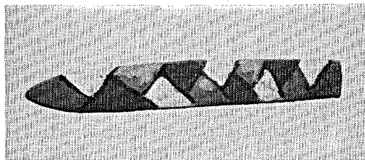
Figures 9a, 9b, 9c: Boomerang and firesticks illustrating three possible 3-colorings of a strip. (James Cook University, Material Culture Unit. 9a: No. AAB 79.1.371; 9b: No. AAB 79.1.132; 9c: No. AAB 79.1.345).
