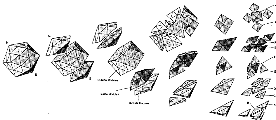
Figure 2: Synergetic modules
