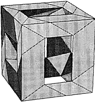
Figure 7: A regular hexahedron which inscribes a dodecahedron
