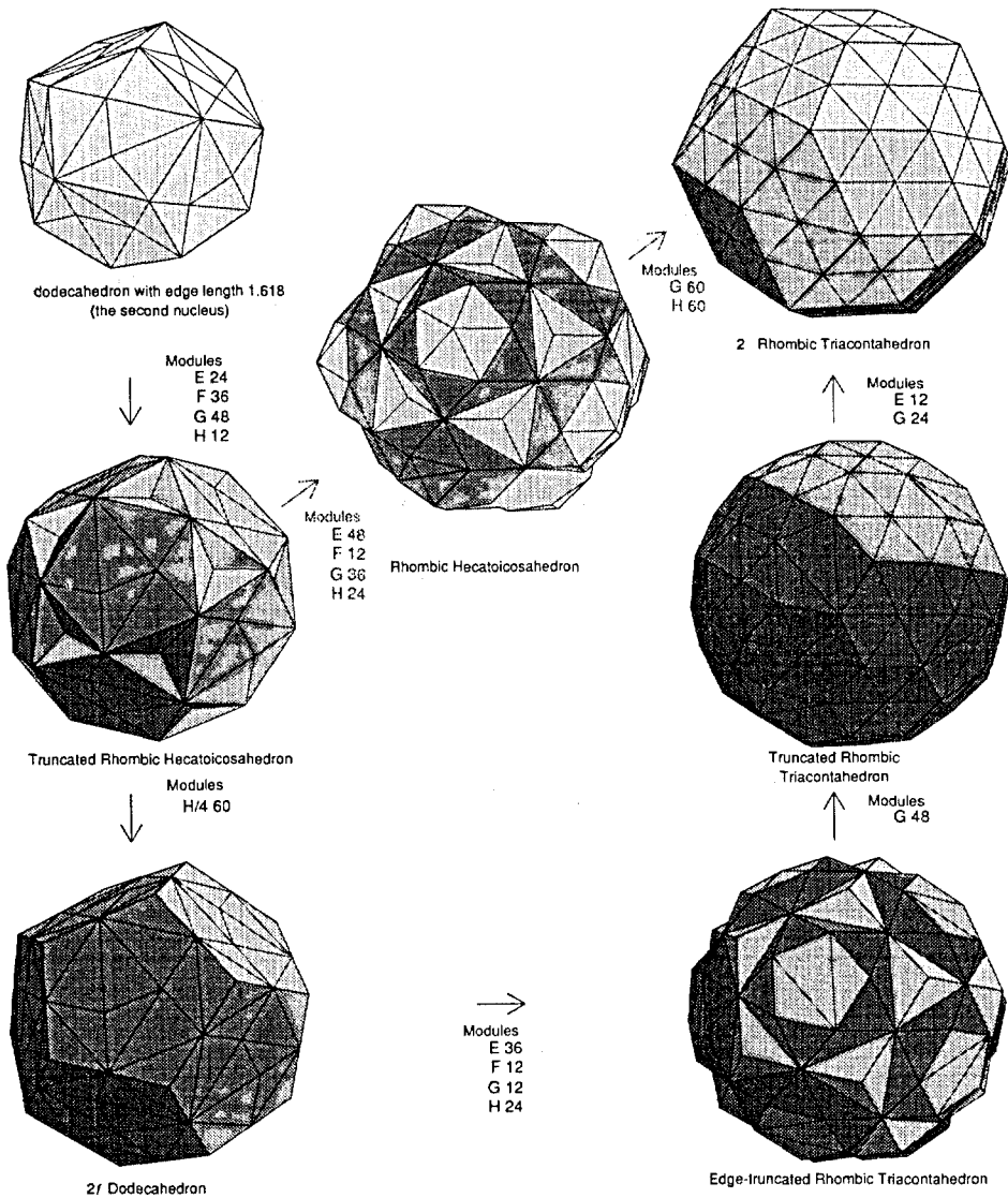
Figure 4: Rhombic triacontahedron
