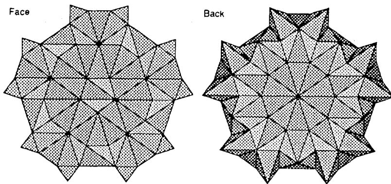
Figure 6: Tiling
