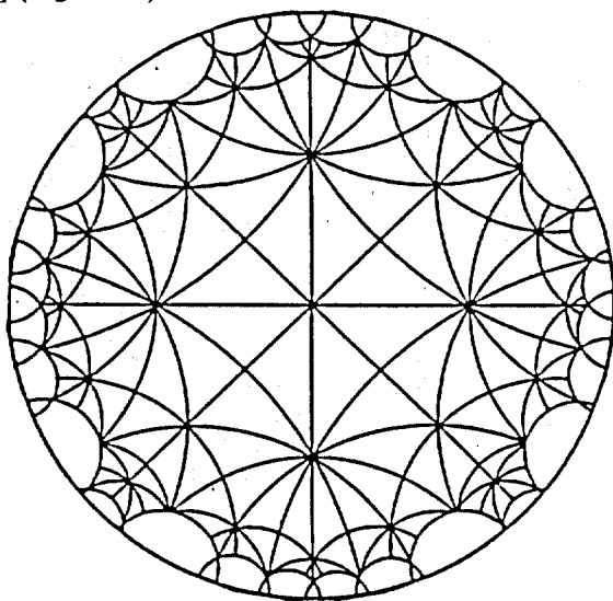
Figure 16: Tessellation [4, 6]
