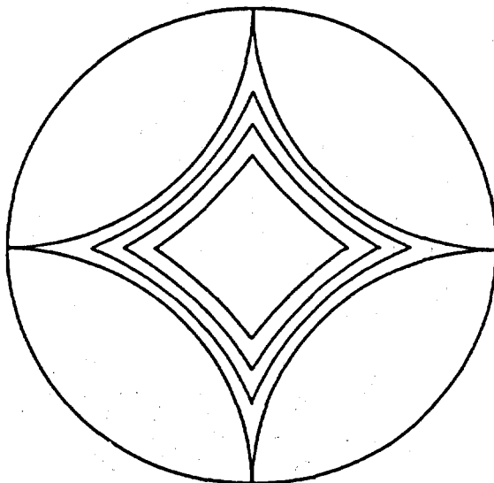
Inside to out, q = 5, 6, 8, \infty with angle 72^\circ, 60^\circ, 45^\circ, 0^\circ respectively
