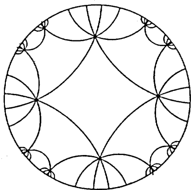
(c) [4, 8]
