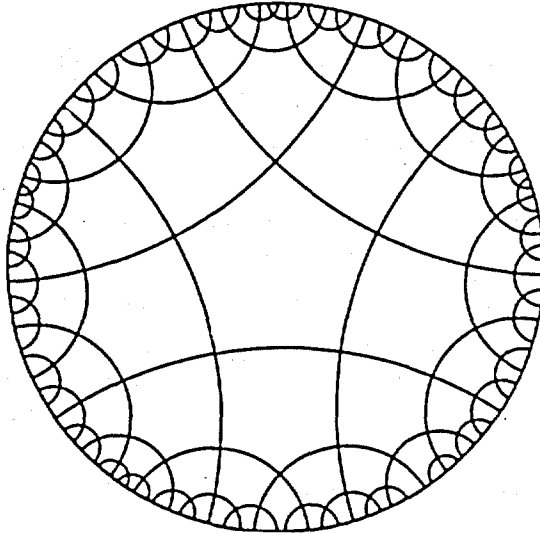
(a) [5, 4], Pentagons
