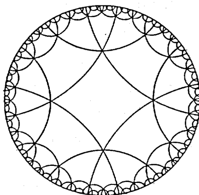
(b) [4, 6]
