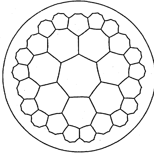
(b) [7, 3], Septagons
