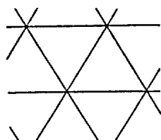
(a) [3, 6]
