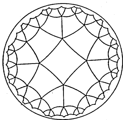
(a) [4, 5]
