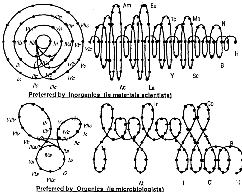
Figure 2: Two periodic tables.
