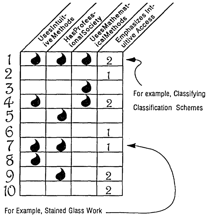
Figure 4: A table view of the lattice relationships.
