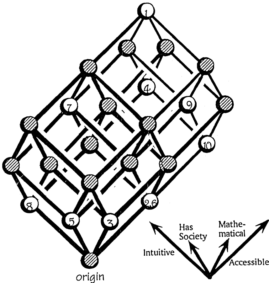
Figure 3: A simple concept lattice.
