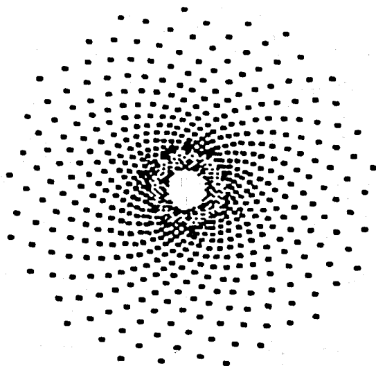
Figure 1.3: Points equally spaced along the logarithmic spiral r = e^{k\theta} ( k = 1/800 ) at intervals of 360^\circ/\varphi^2 appear to form 21 secondary spirals in one direction and 34 in the other.
