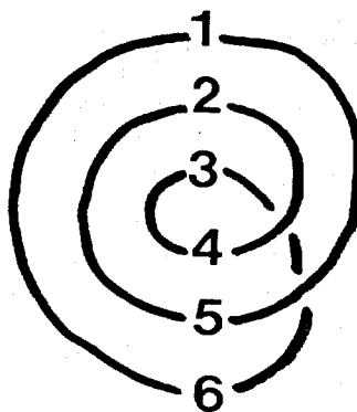
Figure 2.3: The spiral symmetry of the sestina.
