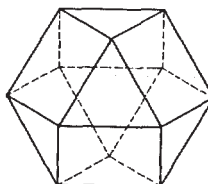
Figure 1: Cuboctahedron
