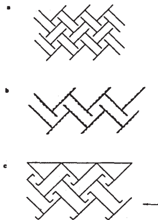
Figure 6: Analyzing Figure 1 a. Primary line work of Hohokam precursors to Figure 1. The pattern of line work belongs to symmetry group pgg. b. The method of adding elaborative detail to the line structures in Figure 6a. c. Initiation and cutoff levels of Figure 1.
