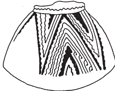
Figure 11: The decoration synthesized from the fragments of Figure 10.
