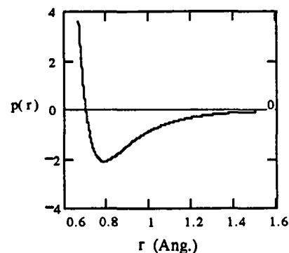
Figure 7. Leonard-Jones Potential formula
