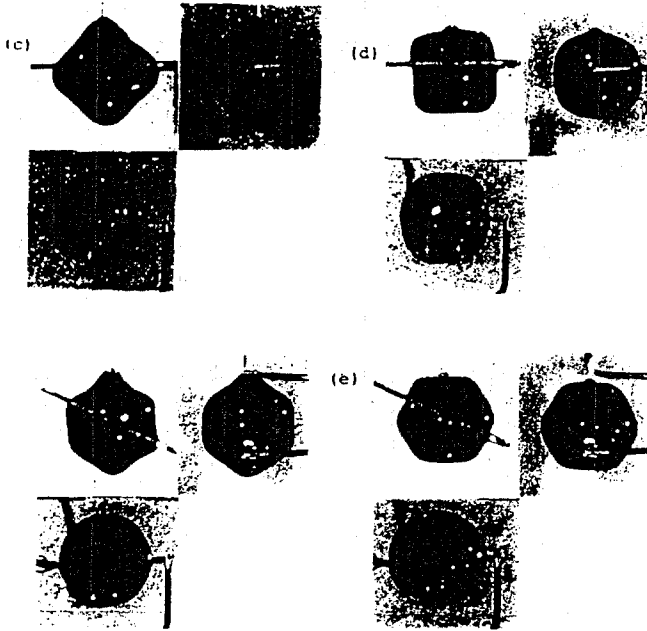
Fig.2 Instantaneous shapes of a drop excited at two surface points. They are similar to the cubic-octahedron and eicosahedron-dodecahedron modes. But, exact coincidences are suspicious.
