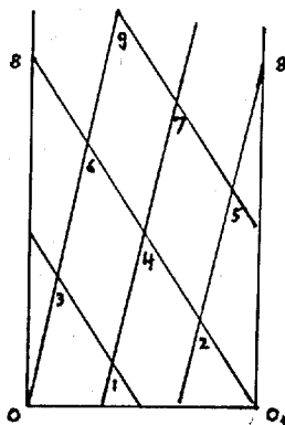
Figure 3: The opposed parastichy pair (2, 3).
