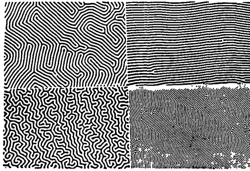
Figure 2 Various equilibrium demagnetized magnetic domain structures ( M=0 in H=0 ) of an epitaxial YIG garnet film in polarized light
