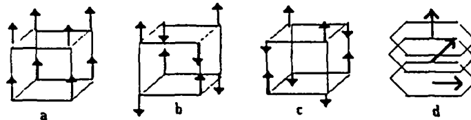
Figure 1 Magnetic ordering: a - ferromagnetic, b - antiferromagnetic, c - ferrimagnetic, d - helimagnetic (the arrows represent the magnetic moments of the atoms in a hypothetical elementary crystal lattice).
