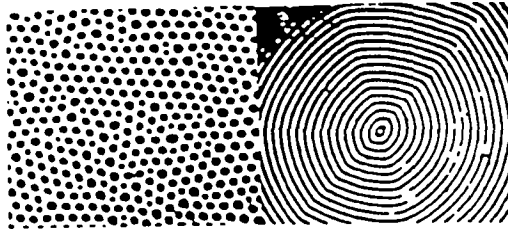
Figure 3 Circular "bubble domains" in an applied dc magnetic field (a), circle domains in a microwave field (b)
