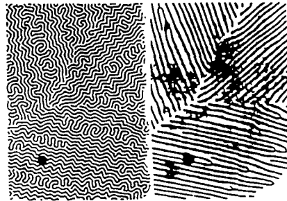
Figure 4 Demagnetized domain structure (a) and domain structure in applied magnetic field (b) of a garnet film on a misoriented (111) substrate
