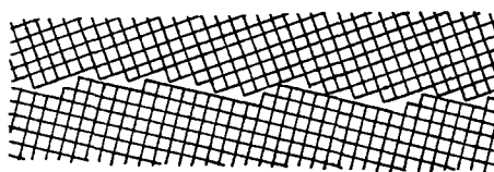
Fig.1: Simplified 2-D model of a grain boundary along which two neighbouring crystal structures form steps against each other. The intersection points of the grids represent atoms or specific groups of atoms.
