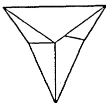
Steffen's TETRADECAHEDRON
