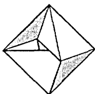
Bricard's OCTAHEDRON
