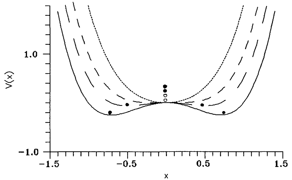
Figure 2: Quartic potentials; a = +1 (dot), 0 (short dash), -0.5 (long dash), -1 (solid). Heavy dots at stable minima, circles at unstable maxima.
