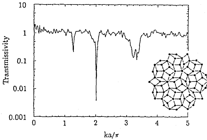
Figure 2: Transmission spectrum of third sound in the Penrose lattice.
