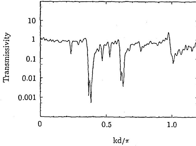
Figure 1: Transmission spectrum of third sound in the Fibonacci lattice.
