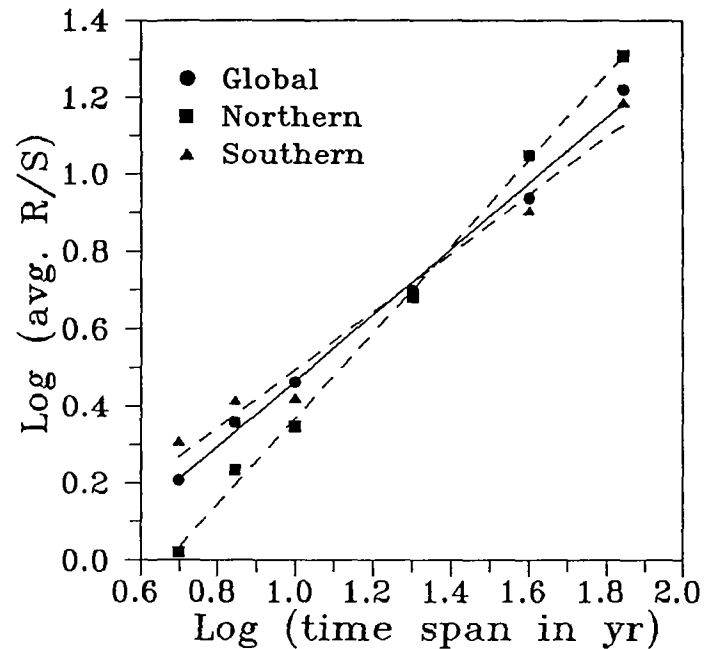
Figure 3: Plot of average rescaled range ( R/S ) values versus time spans for surface air temperature.
