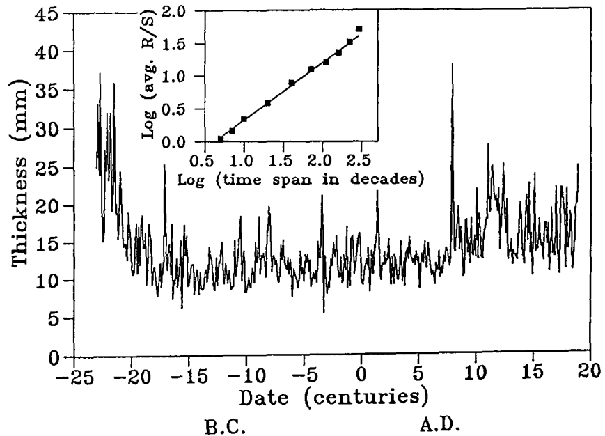
Figure 1: Mean thickness (mm) of the yearly mud layers by decades in lake Saki, Crimea, diagram. Plotted line represents a linear regression line for time spans of 50, 70, 100, 200, 400, 700, 1100, 1600, 2200, and 2900 years.
