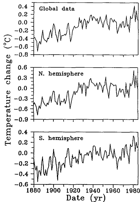
Figure 2: Surface air temperature change estimated from meteorological station records (by data from Hansen and Lebedeff, 1989).
