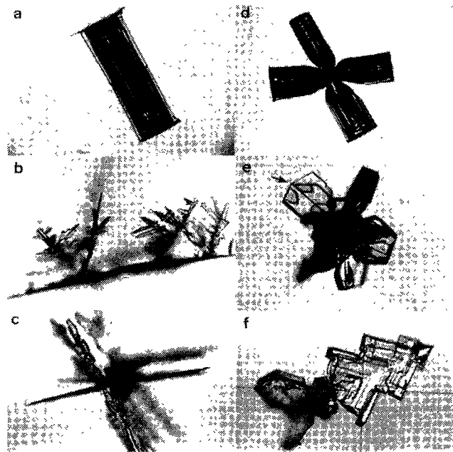
Fig. 2 A variety of snow polycrystals: (a) twin prisms, (b) spatial dendrite, (c) radiating dendrite, (d) combination of bullets, (e) crossed-plates, and (f) peculiar-shaped crystal.
