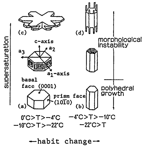
Fig. 1 Schematic representation of variation of growth patterns of single snow crystals with growth conditions (temperature and supersaturation).
