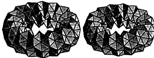
Figure 3: A flat torus with skew-antiprismatic symmetry.
