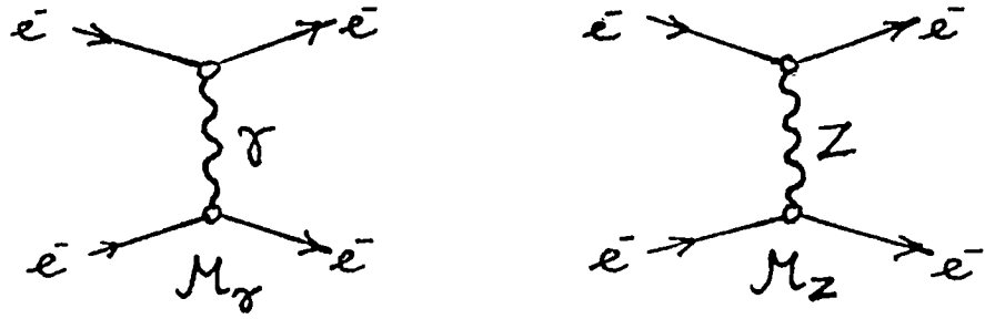
Figure 4: Photon and Z exchange graphs of the e^+e^- \rightarrow e^+e^- process
