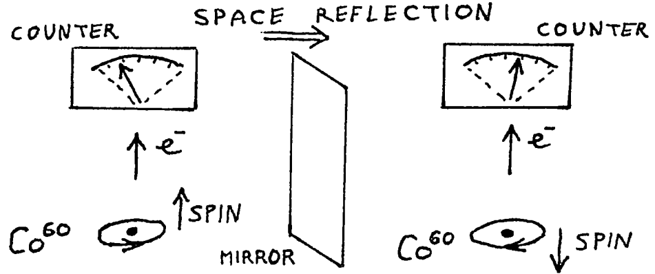
Figure 1: Co^{60} experiment.
