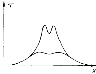
Fig.1 Complex heat structure with two maxima.
