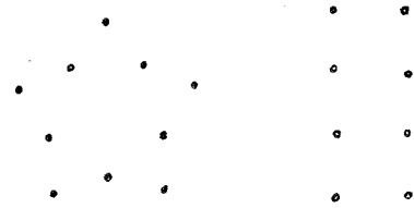
Fig. 2. Examples of configurations of maxima in 2-D complex heat structures.
