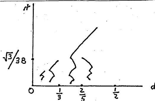
Fig. 4. Vortices in the (d,r) plane. (Schematic diagram)
