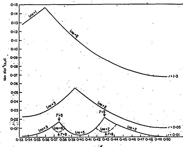
Fig. 3. min dist 2 (0,n) as a function of d when T=5 and T=8 . (Lno = leaf nearest zero.)
